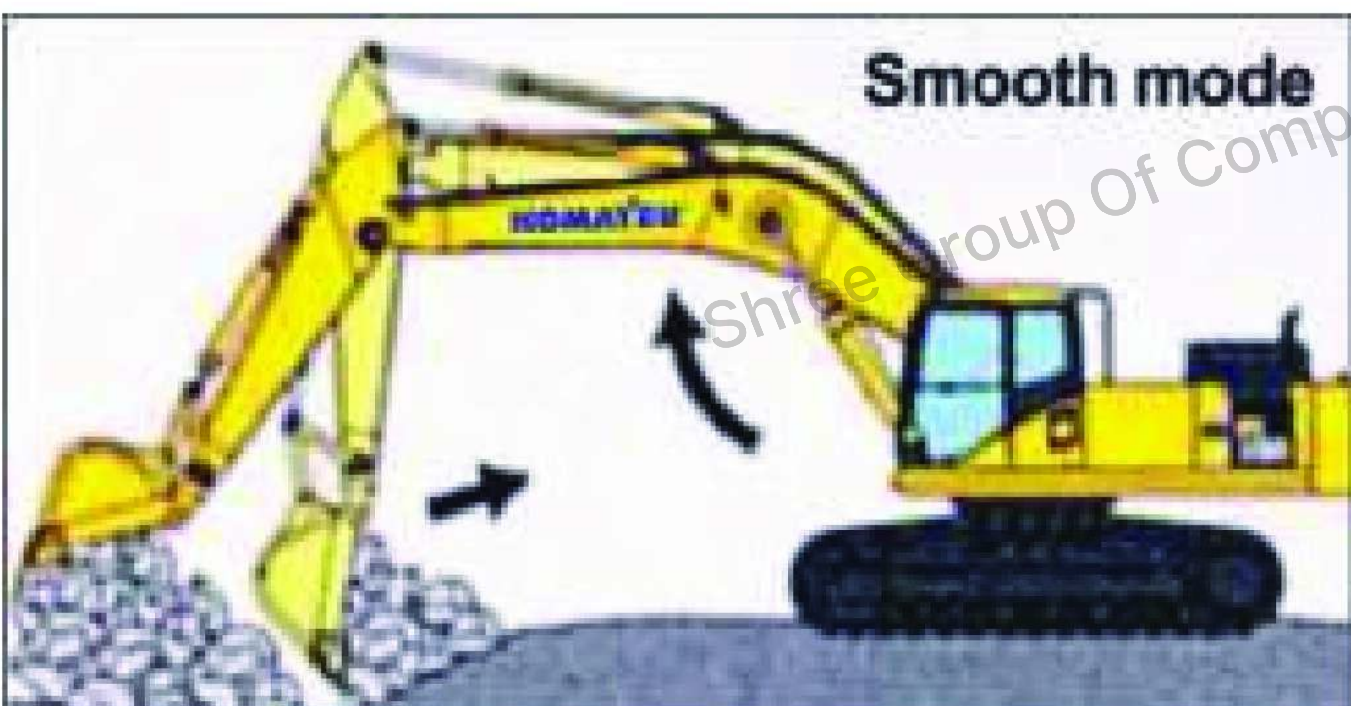
Boom floats upward, reduced lifting of machine front. This facilitates gathering blasted rock and scraping down operations.
